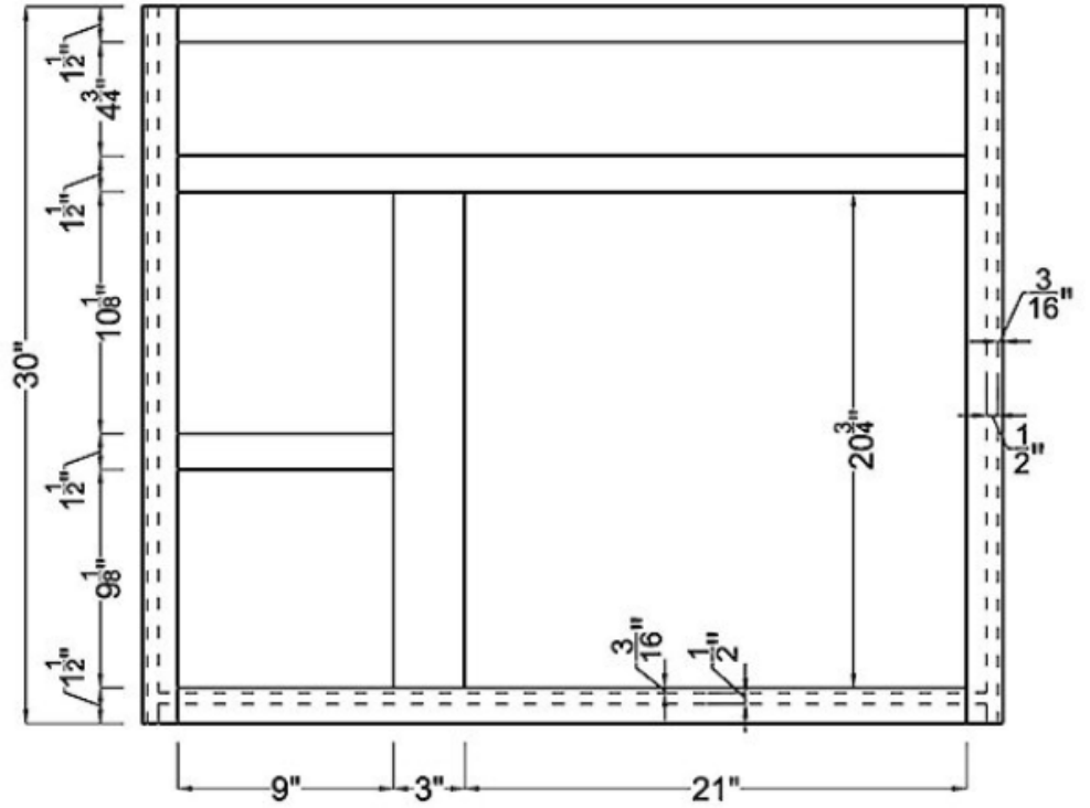
Frame
