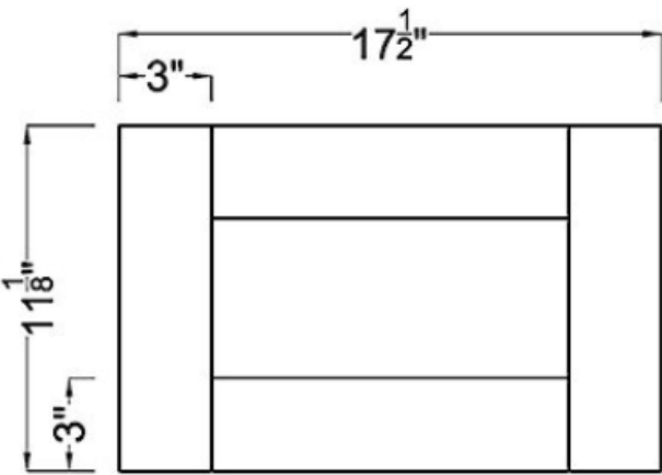
Drawer Front ×2
