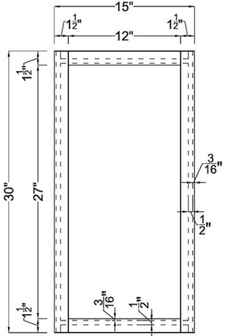
Frame
