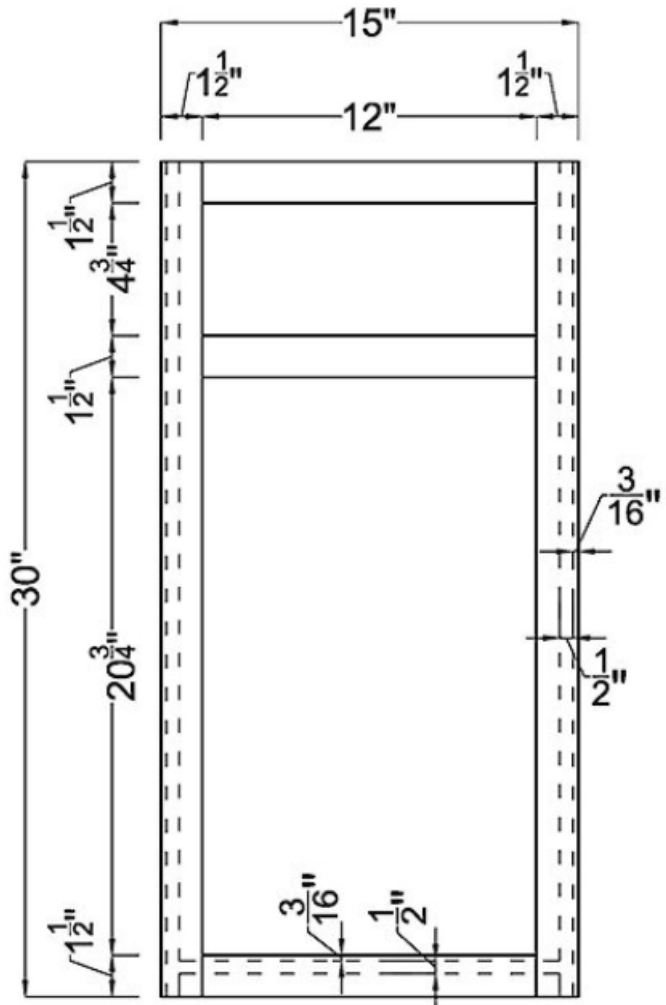
Frame
