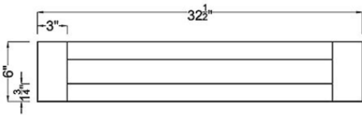
Drawer Front x1
