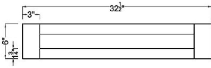
Drawer Front ×1
