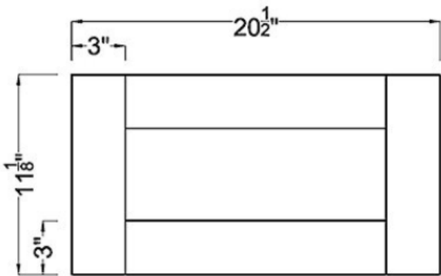
Drawer Front ×2
