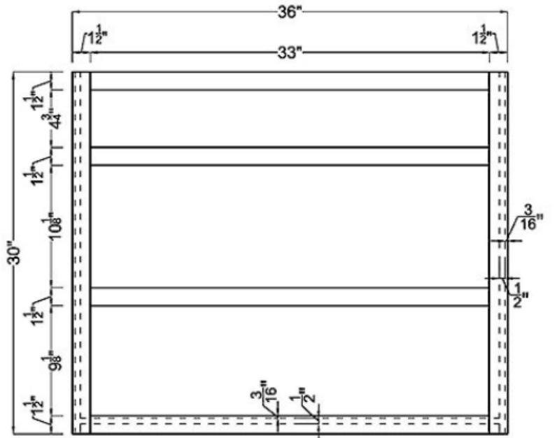
Frame
