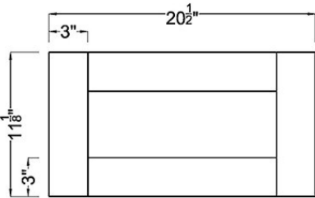
Drawer Front ×2
