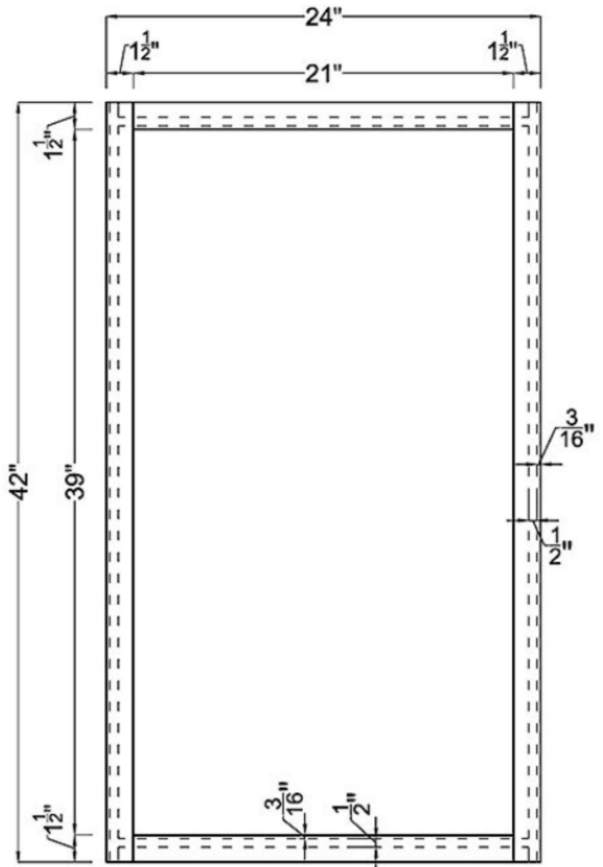
Frame
