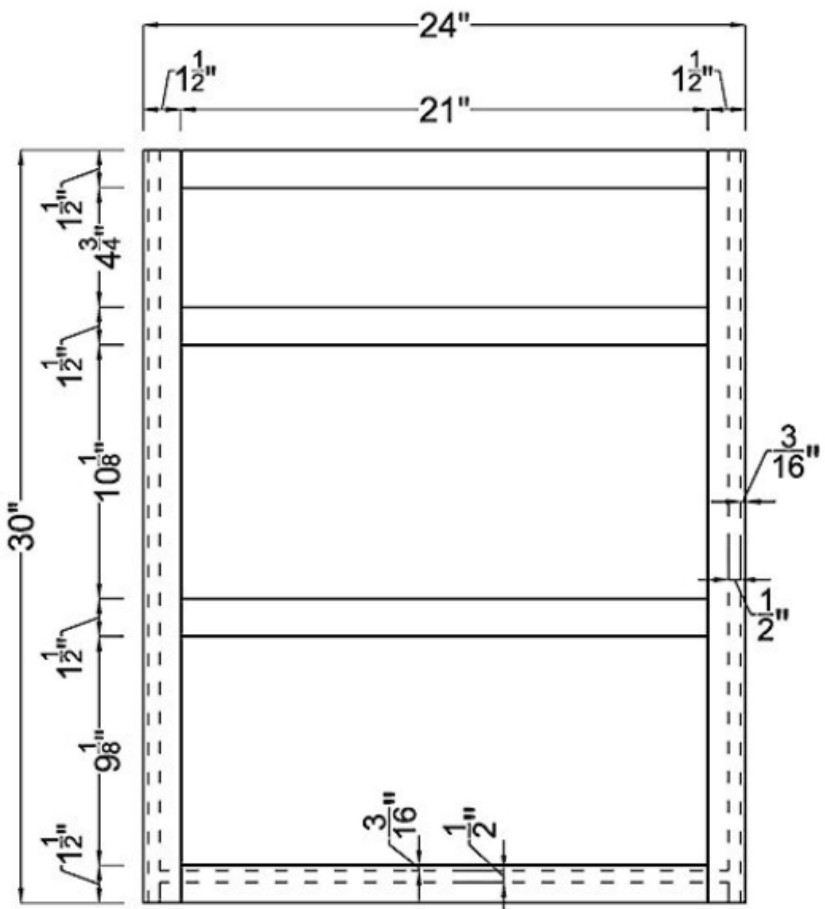
Frame
