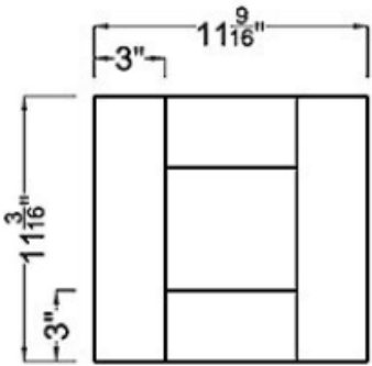
Drawer Front ×2
