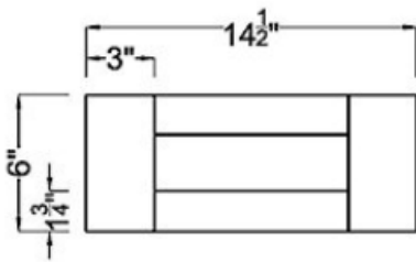
Drawer Front ×1
