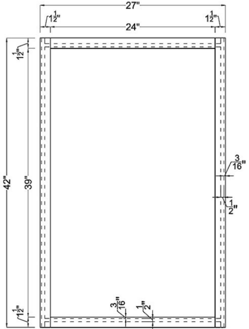
Frame
