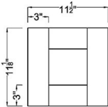
Drawer Front ×2
