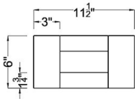
Drawer Front ×1
