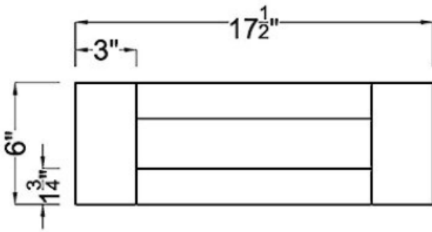
Drawer Front ×1
