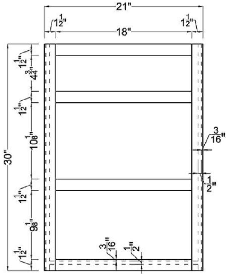
Frame
