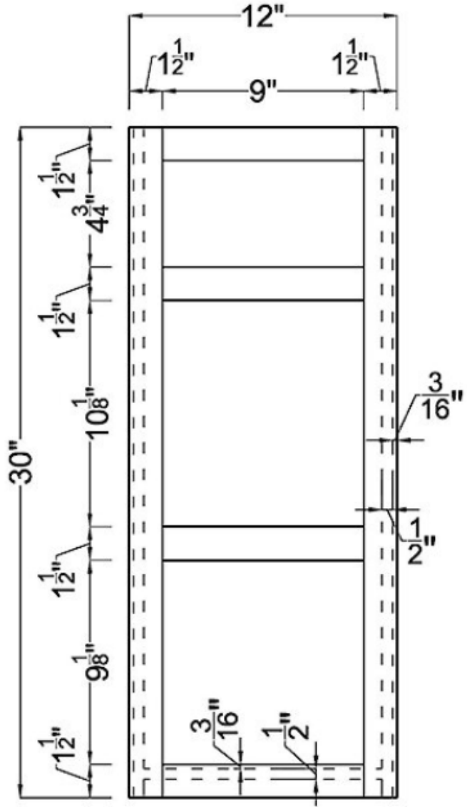
Frame
