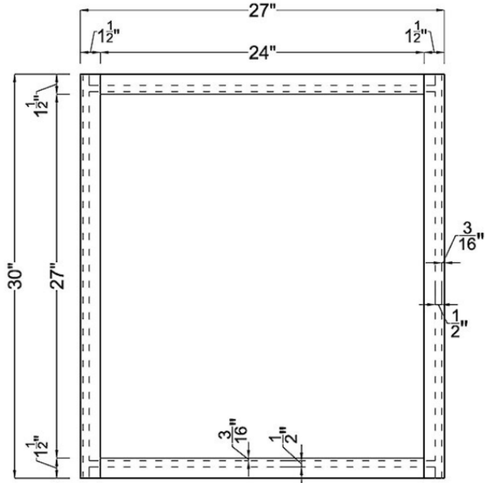
Frame
