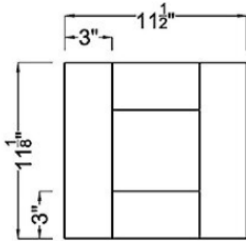
Drawer Front ×2
