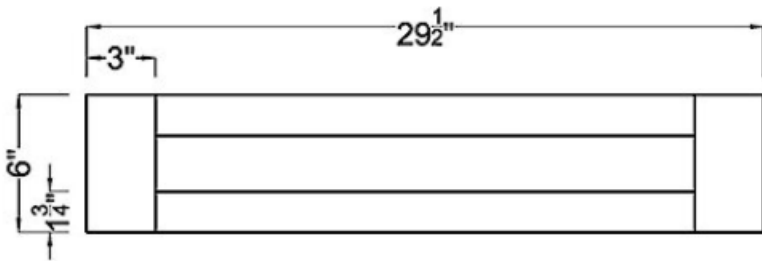
False Drawer Front x1
