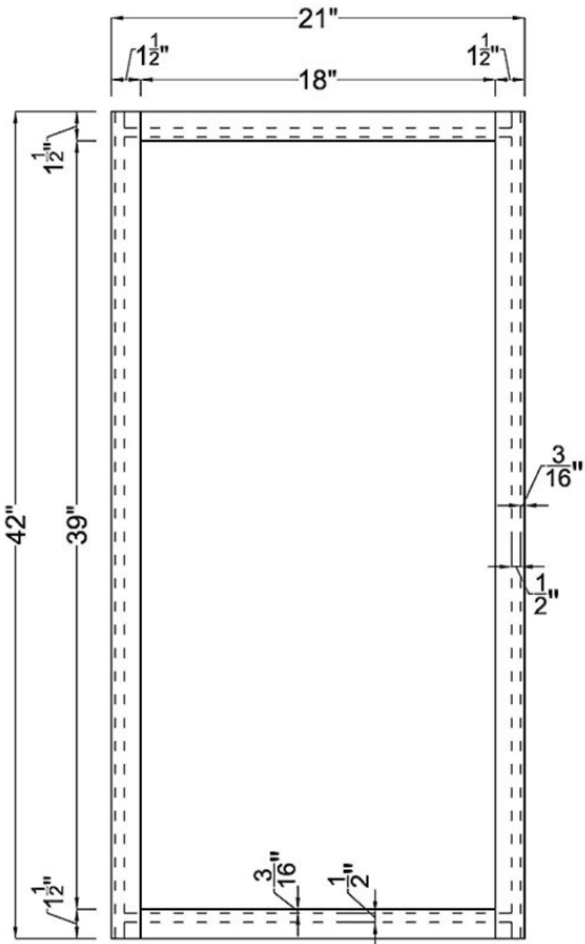
Frame
