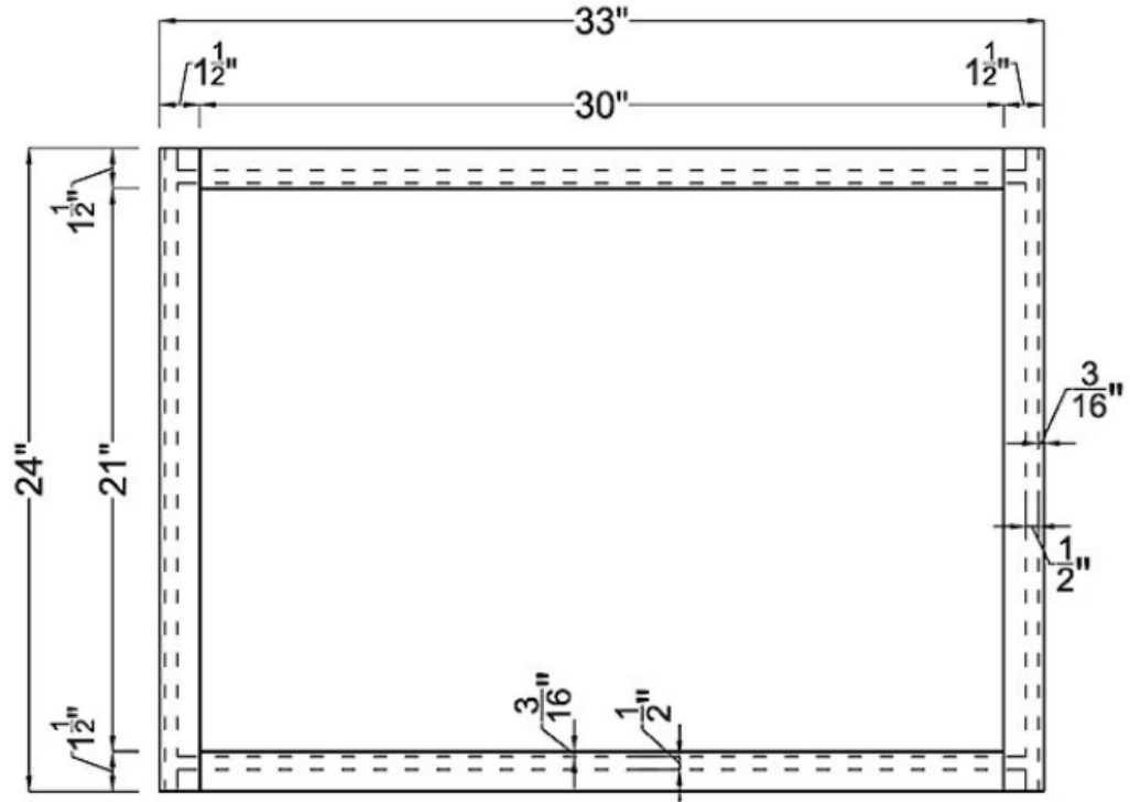
Frame
