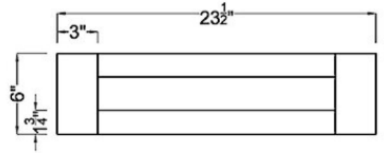
False Drawer Front x1
