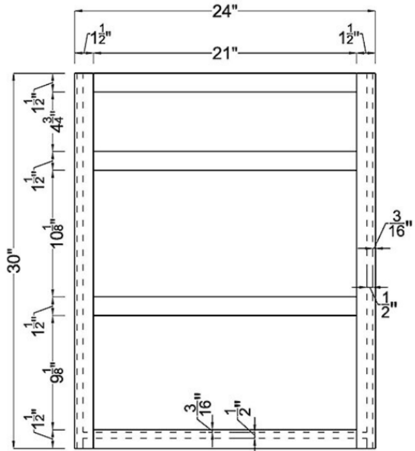
Frame
