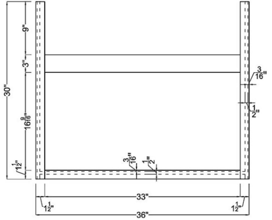
Frame
