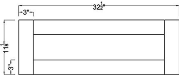
Drawer Front ×2
