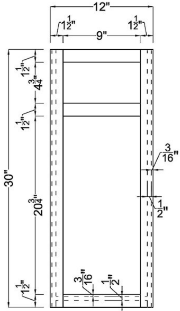
Frame
