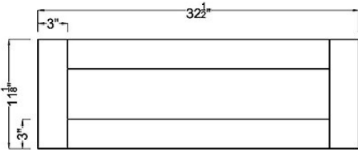
Drawer Front ×2
