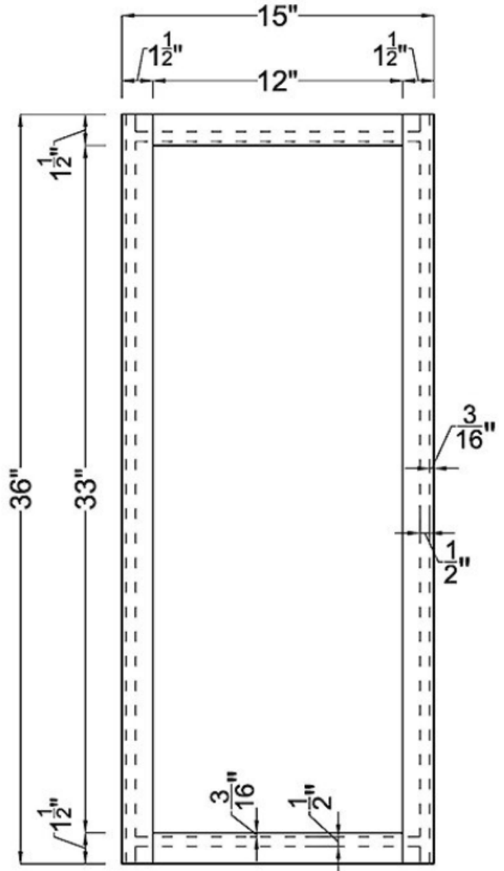
Frame
