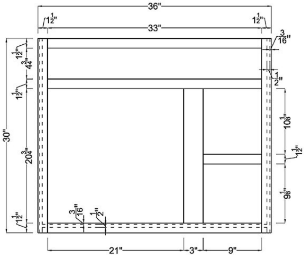
Frame
