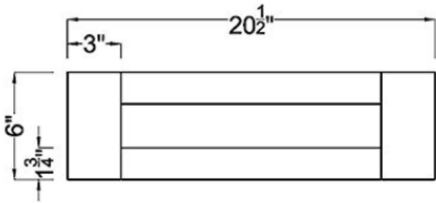
Drawer Front ×1
