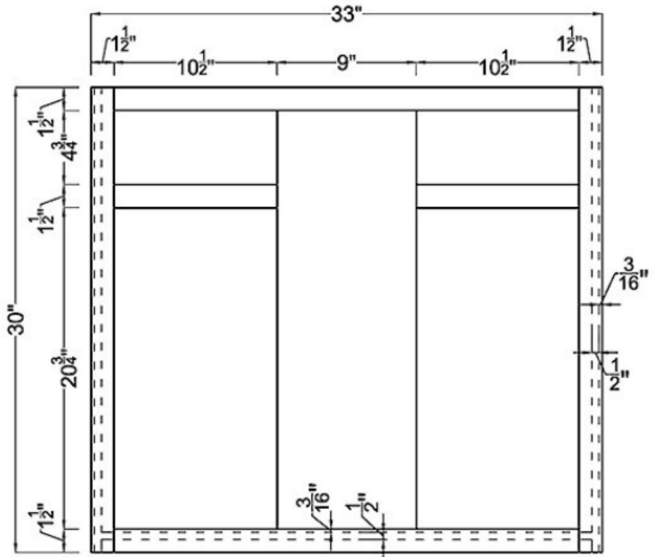
Frame
