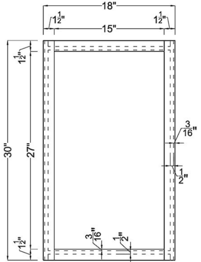
Frame
