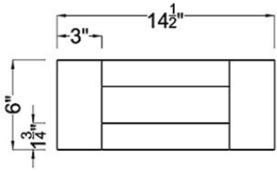
Drawer Front ×1
