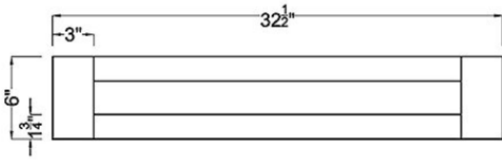
Drawer Front ×1
