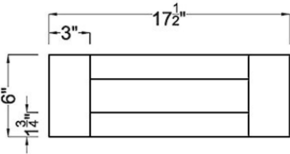
Drawer Front ×1
