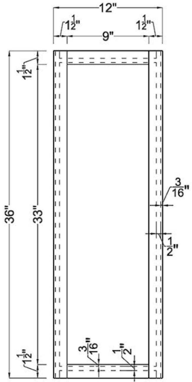
Frame
