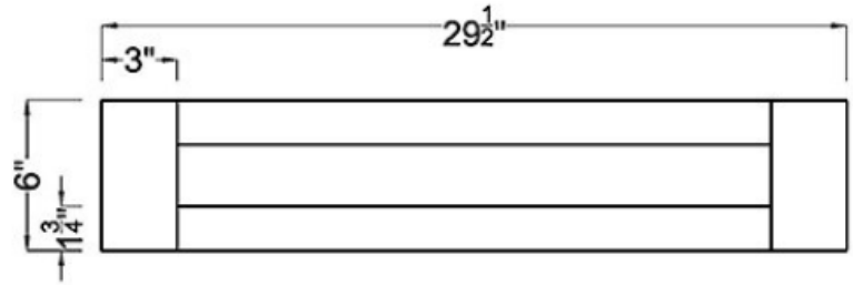
False Drawer Front ×1
