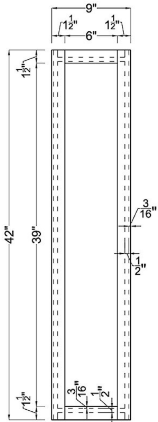
Frame
