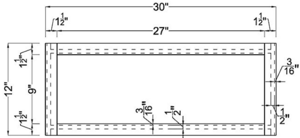
Frame
