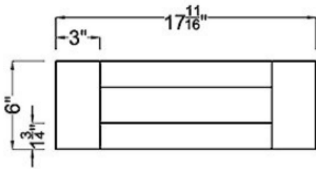
Drawer Front ×2
