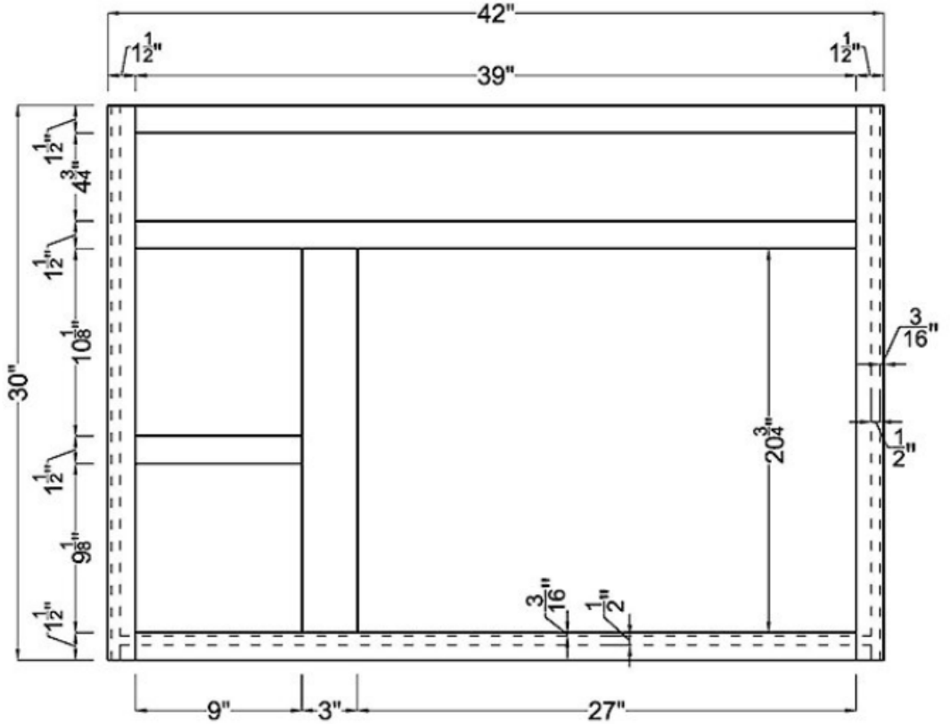
Frame
