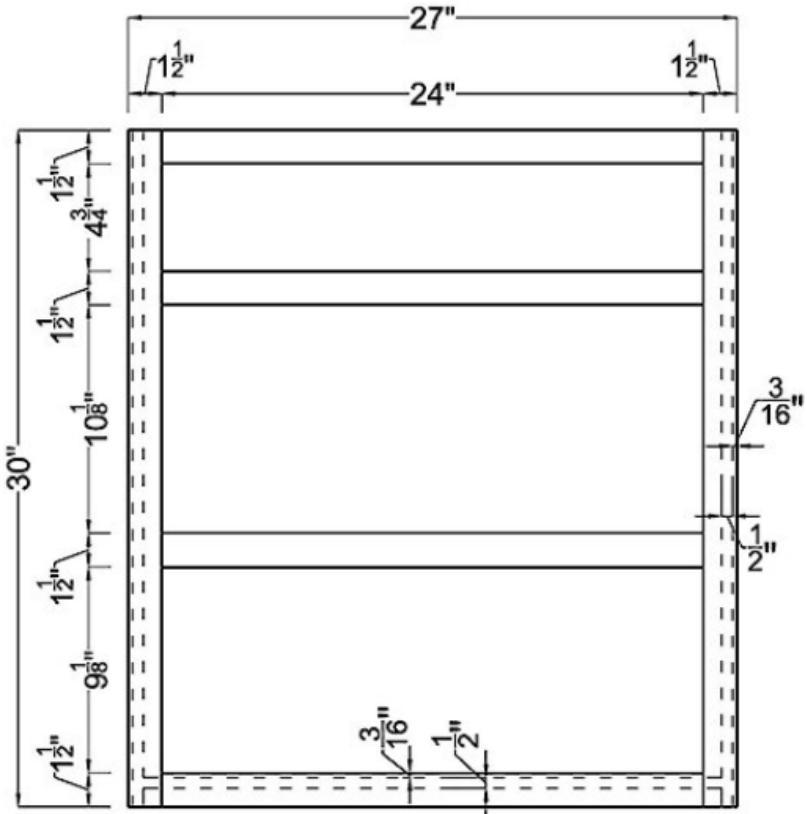
Frame
