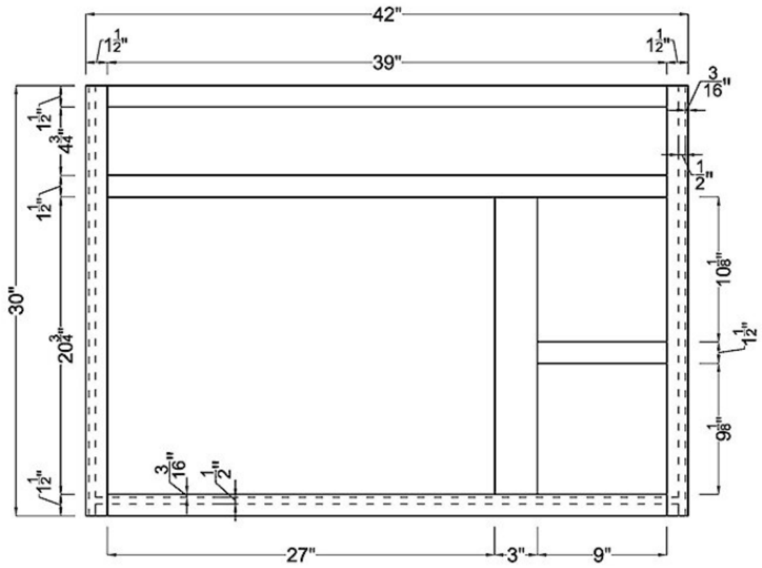
Frame
