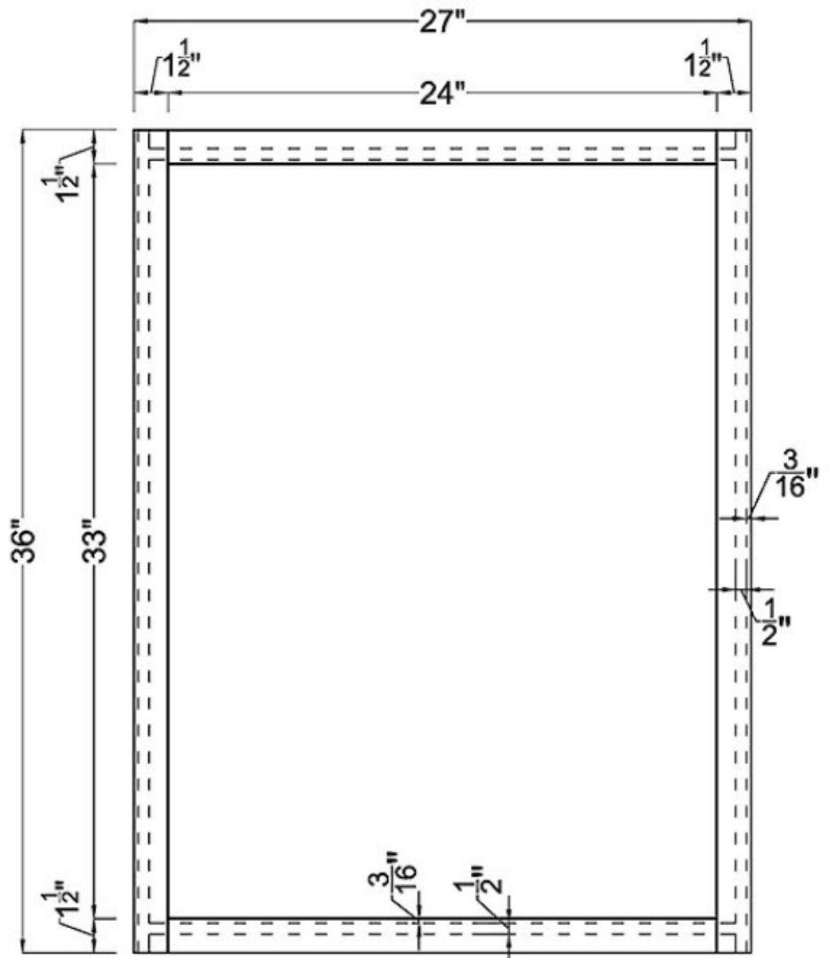
Frame
