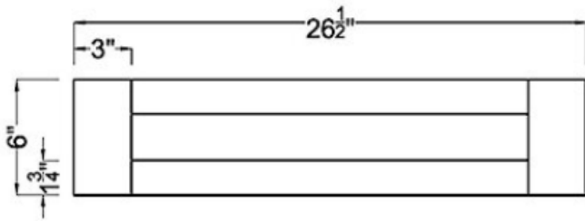
Drawer Front ×1
