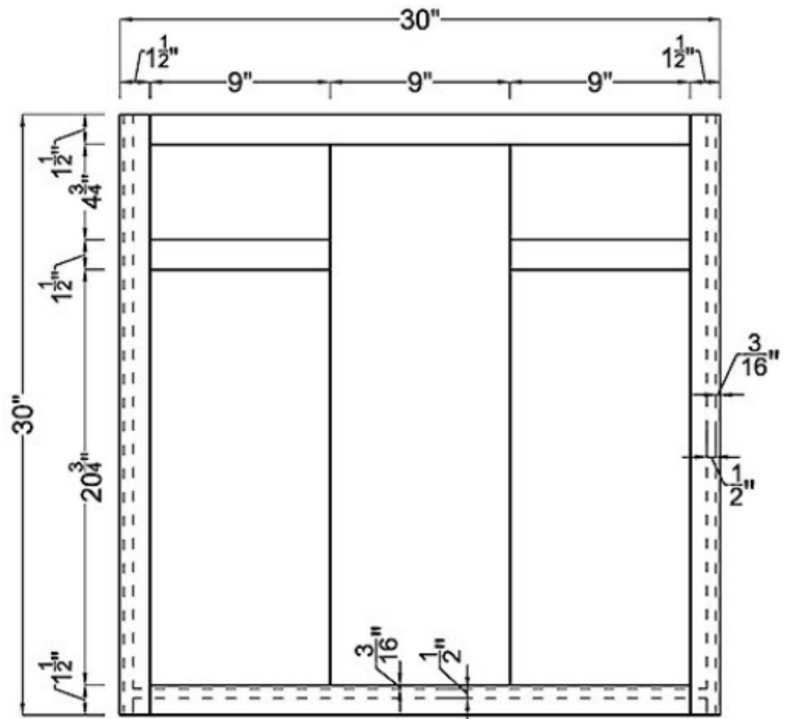
Frame
