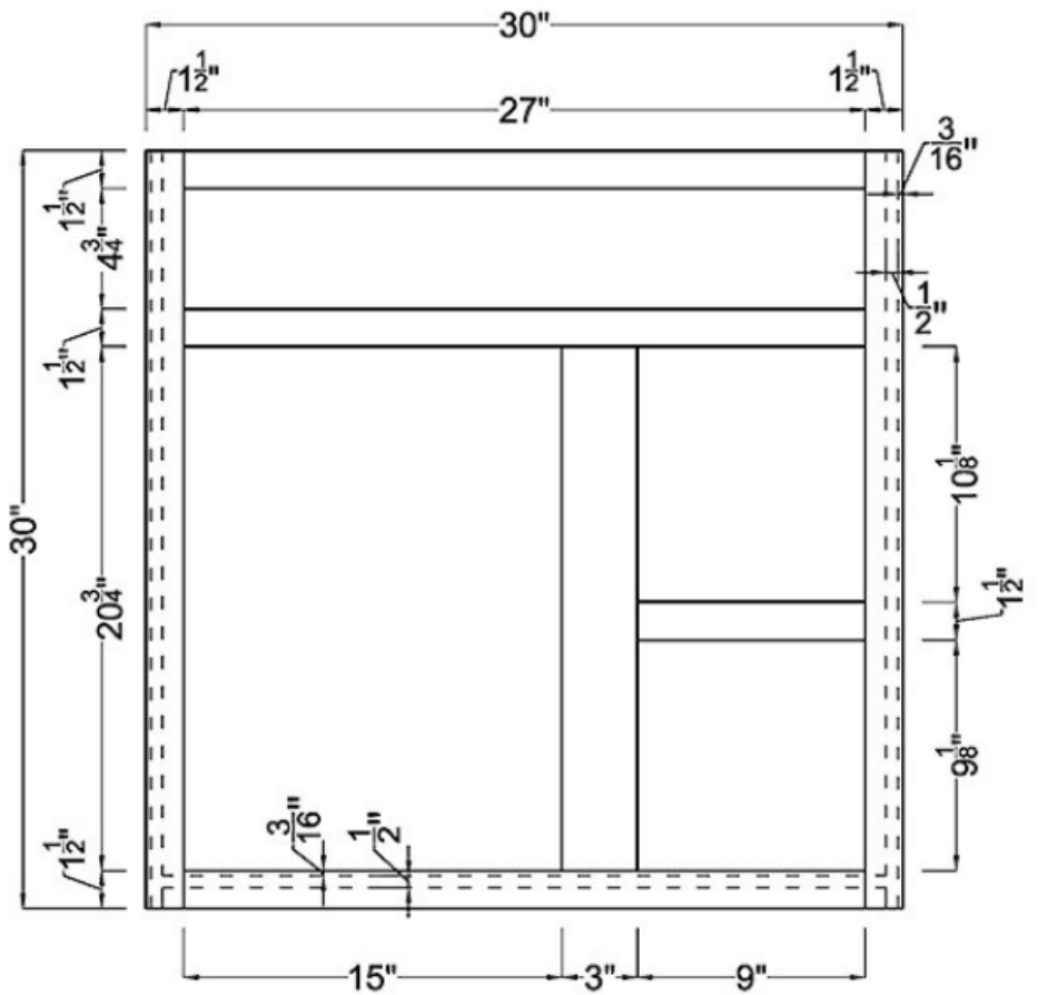
Frame
