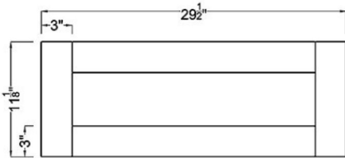
Drawer Front ×2
