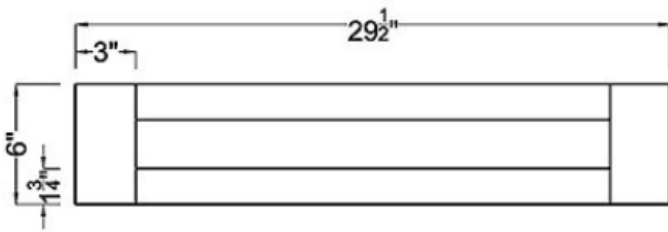
Drawer Front ×1
