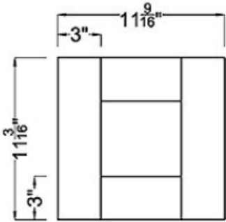
Drawer Front x2
