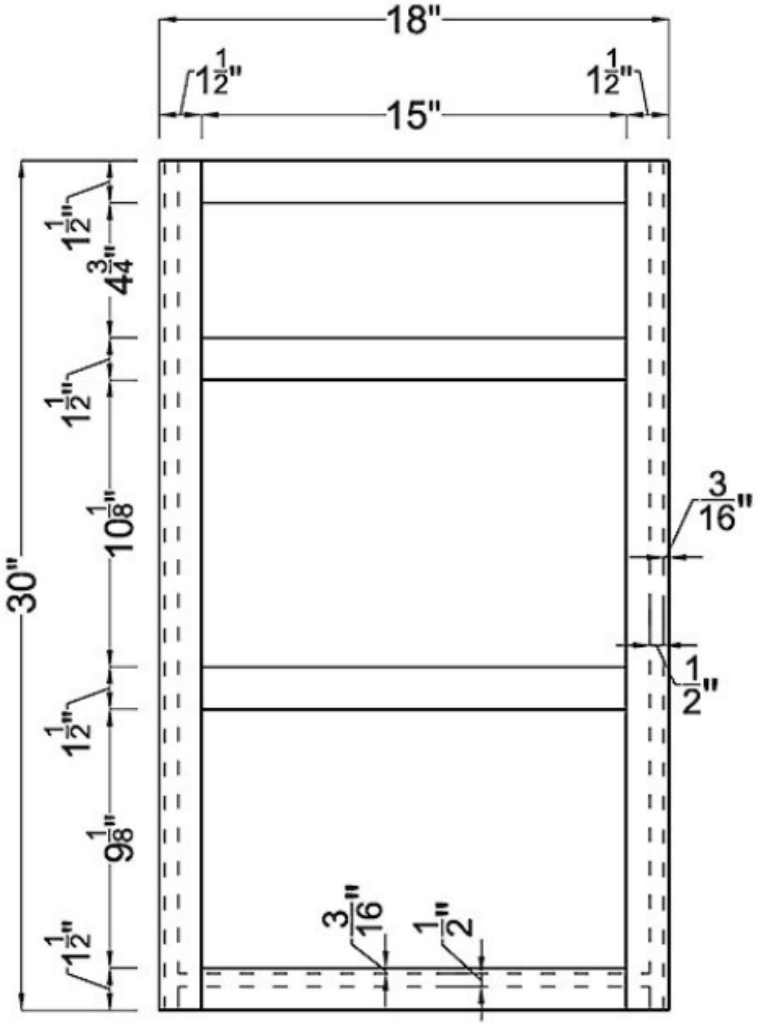
Frame
