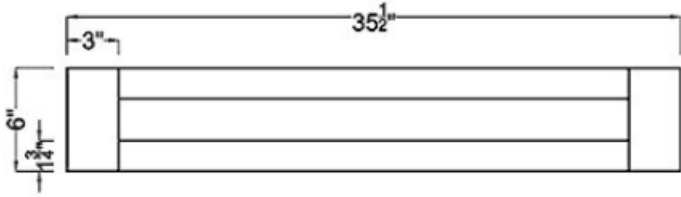
Drawer Front ×1
