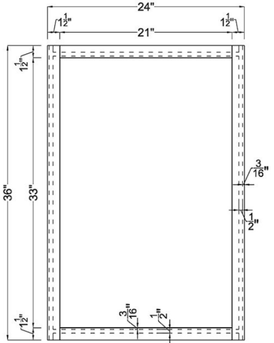
Frame
