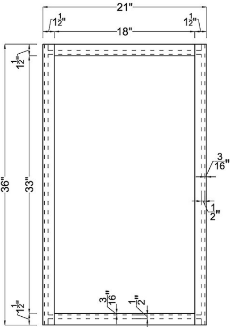
Frame
