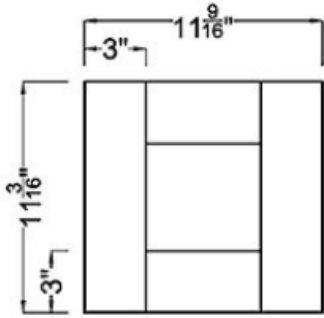
Drawer Front ×2
