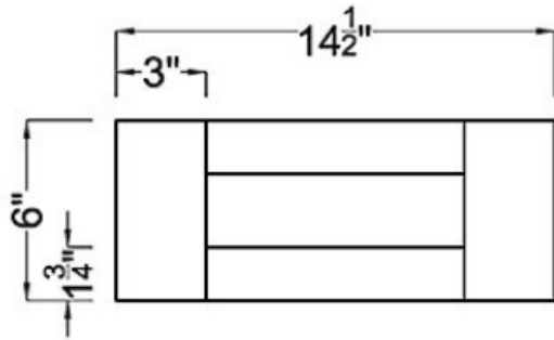
Drawer Front ×1
