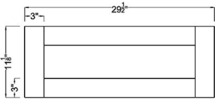
Drawer Front ×2
