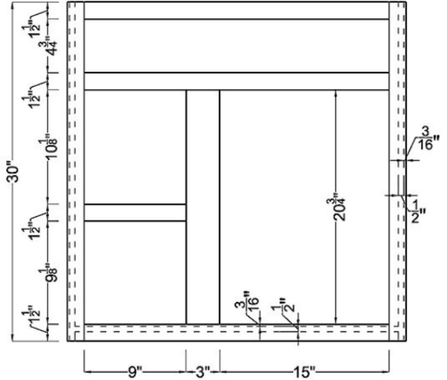
Frame
