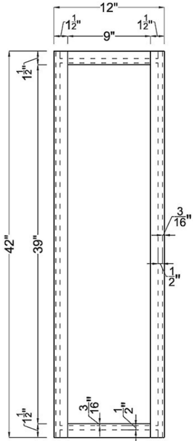
Frame
