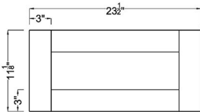
Drawer Front ×2
