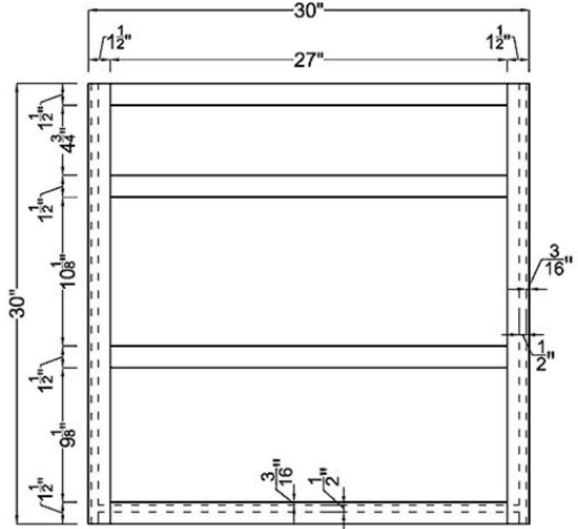
Frame
