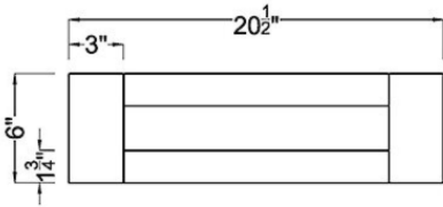
Drawer Front ×1
