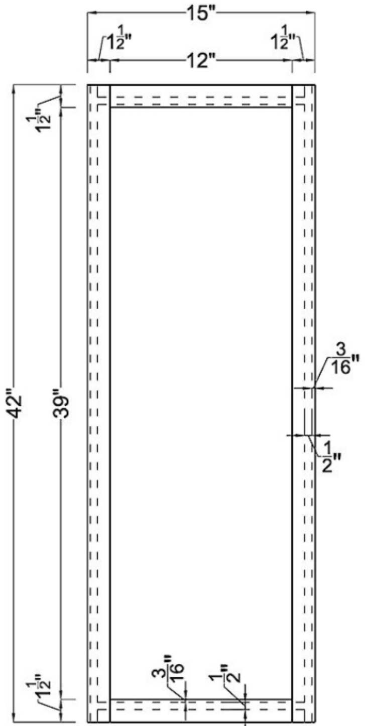
Frame
